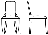
Sedia/chair L89 - cm 51x55x91h
