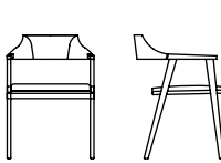
Sedia/chair L30 - cm 53x55x75h
